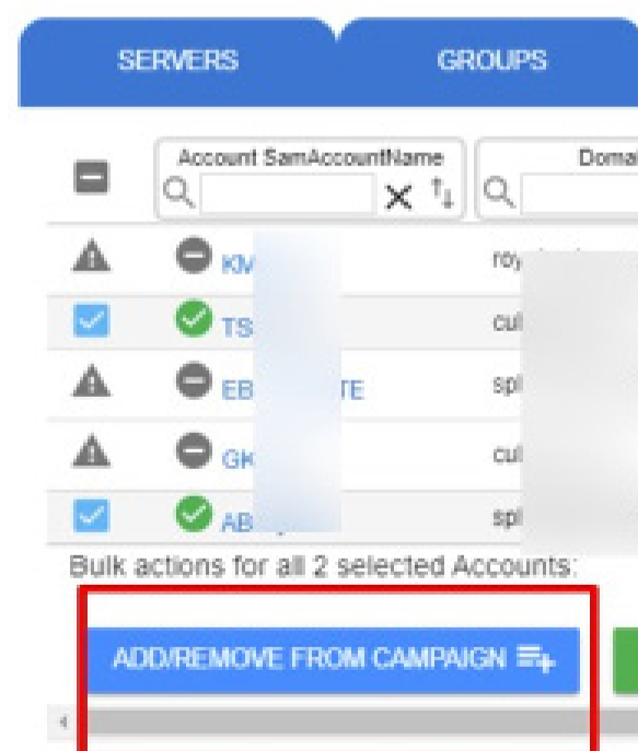
Campaign Toggle
