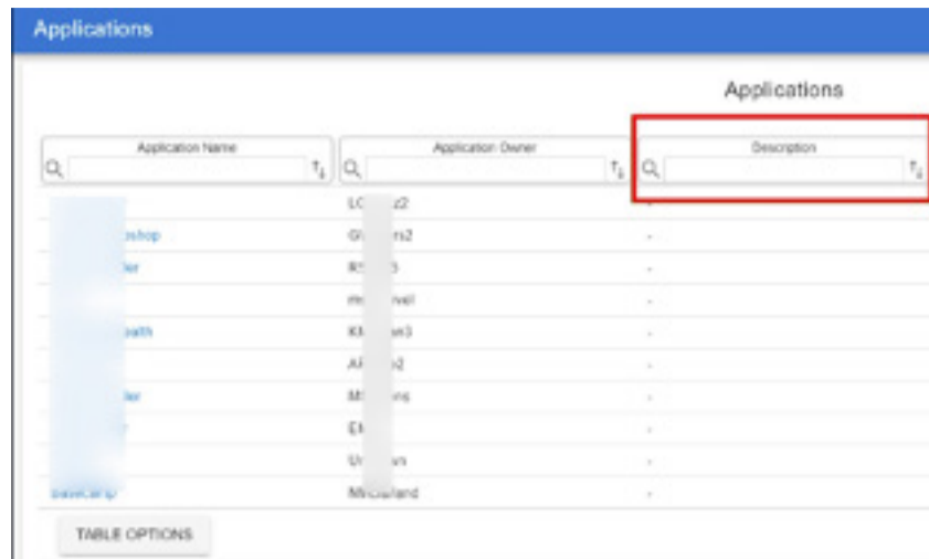
Applications Pane
