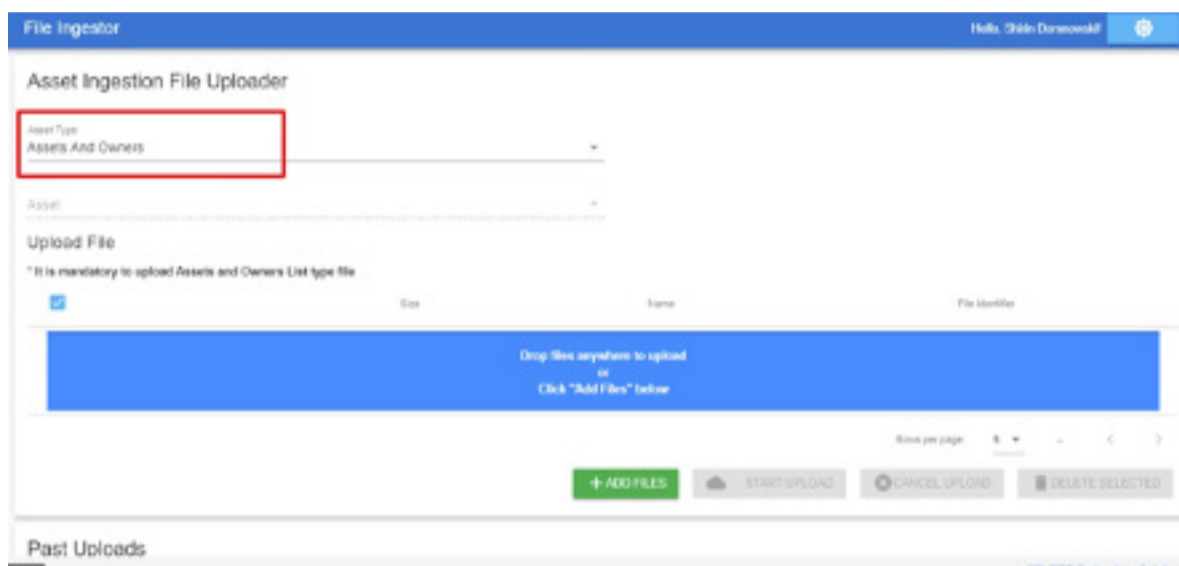
File Ingestor
